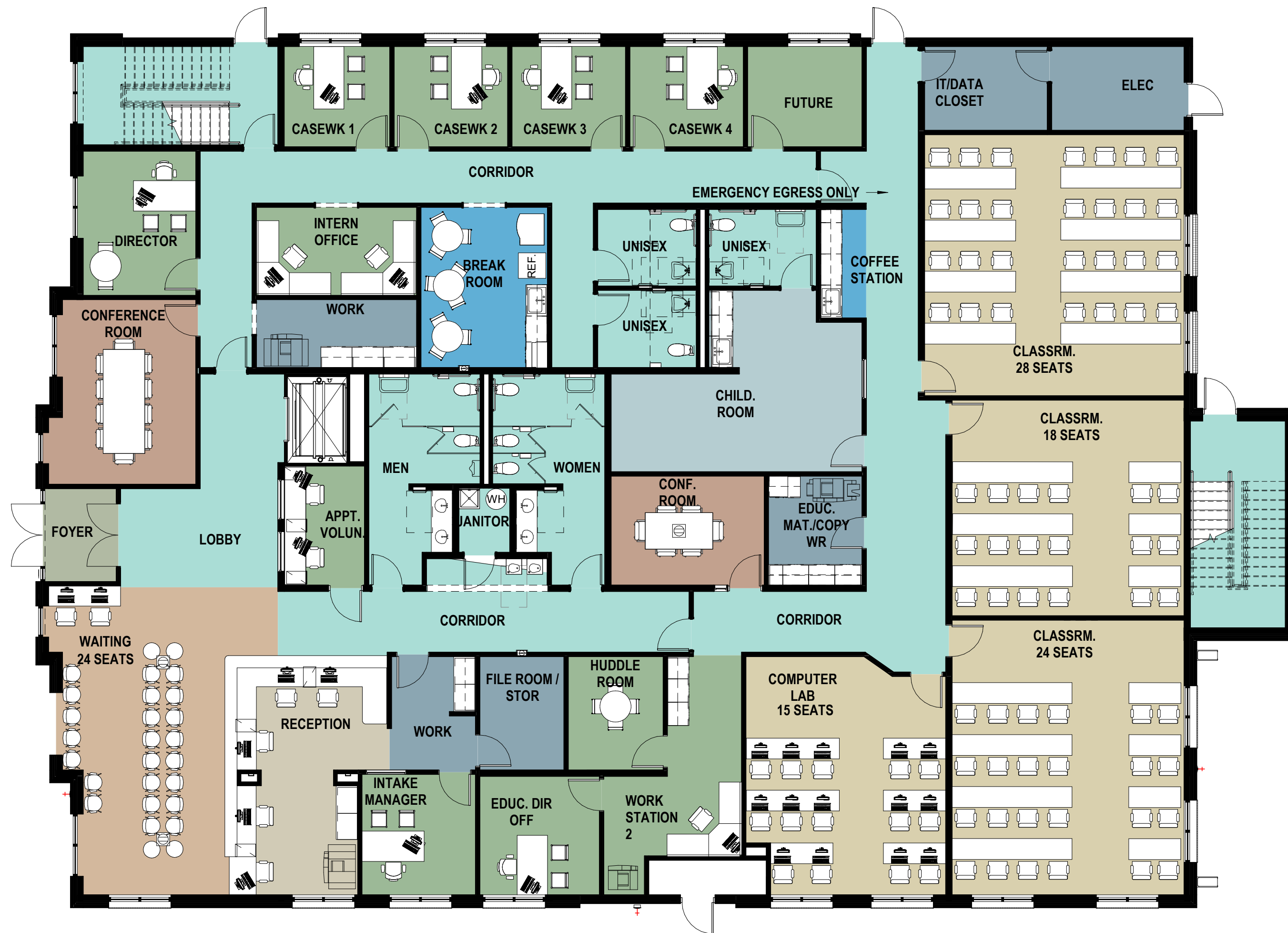
FIRST FLOOR PLAN 1/8" = 1'-0"
